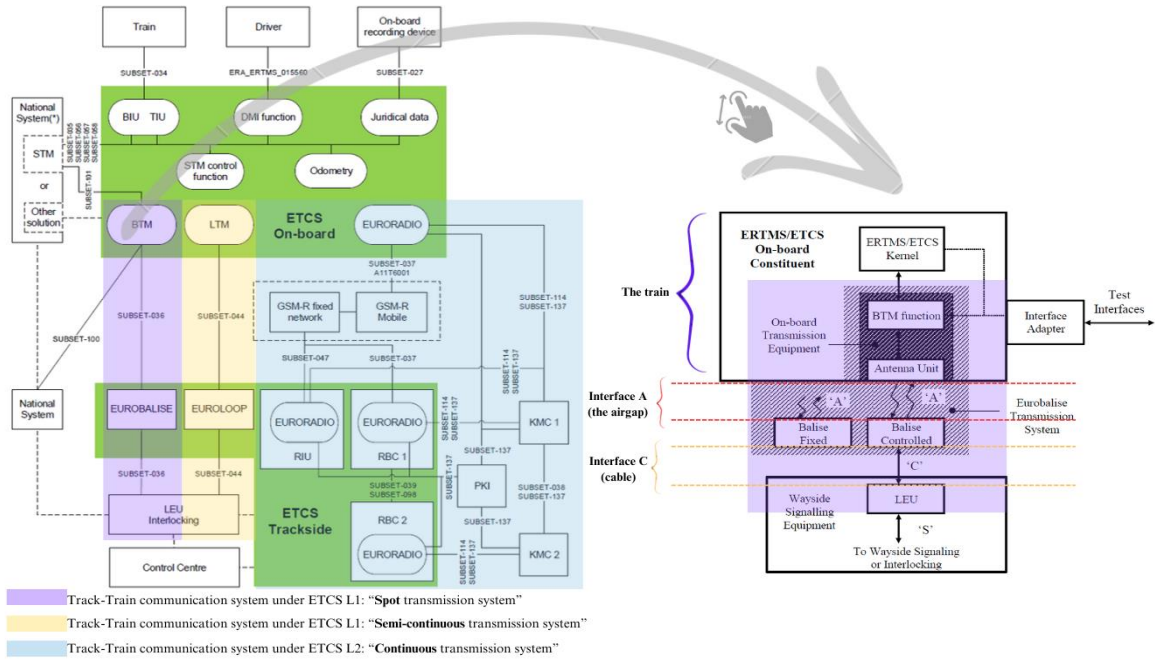
Figure. 1: ERTMS/ETCS system architecture.
